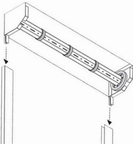
Guide the Box lugs into the Guide Rails.
