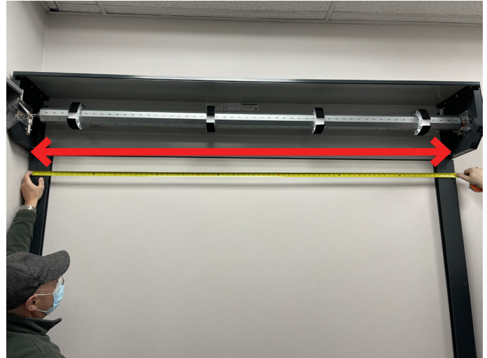
Measuring width of top Guide Rail position.
