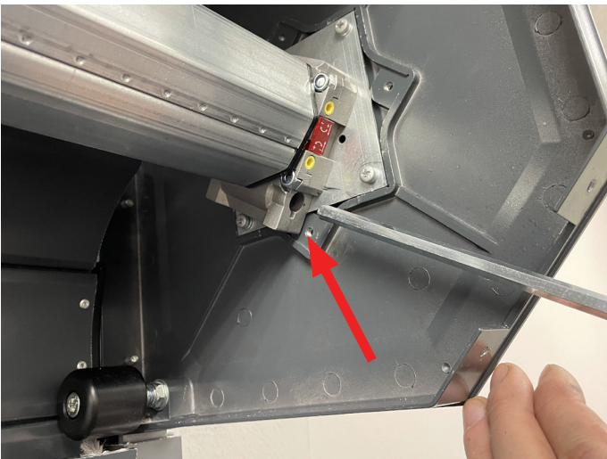
Find the Manual override port below the limit screws.
