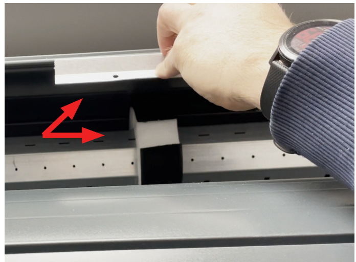
Position Hangers over the Shaft Collars.
